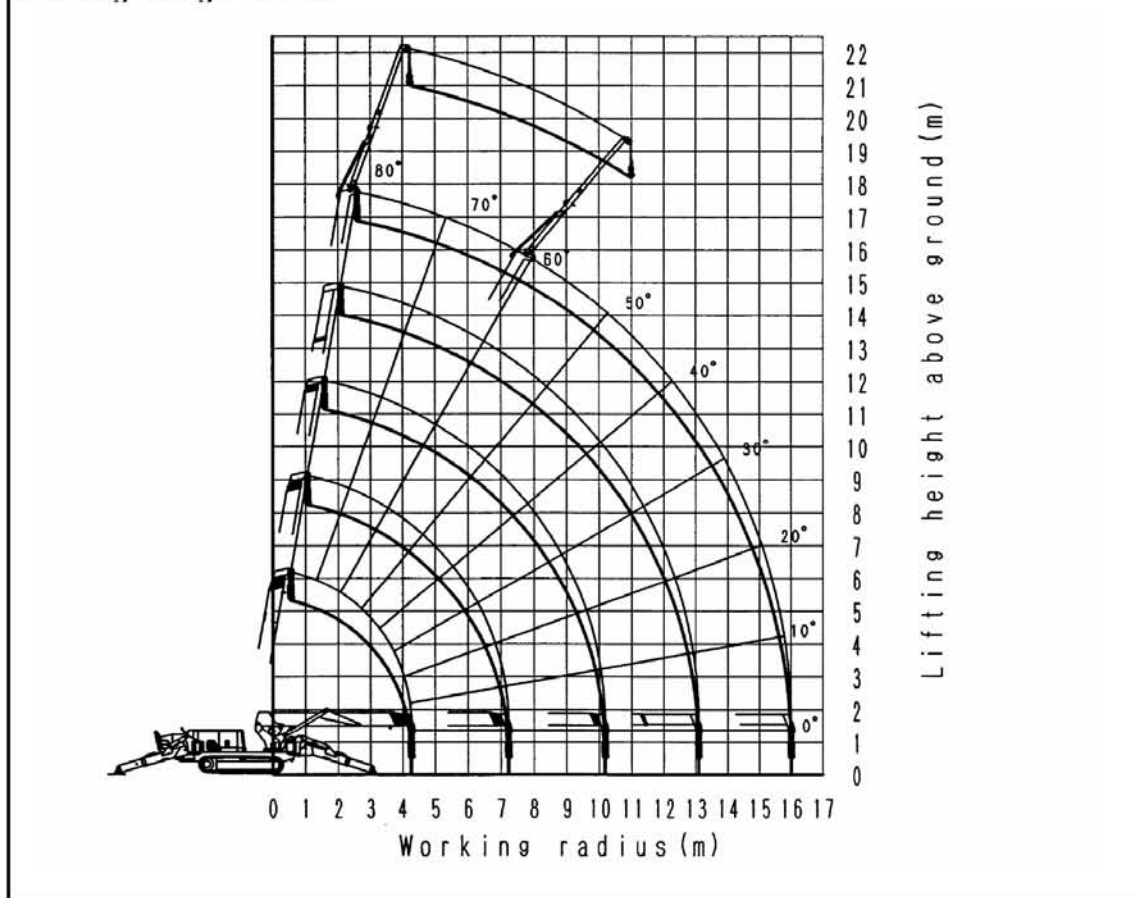
Working Range Chart
